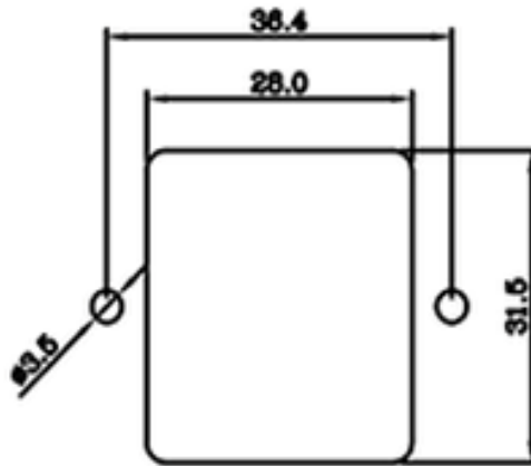
PANEL CUT-OUT
